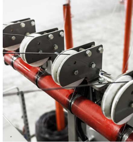
Monitoring of wire breakage and wire end to control the binding wires
