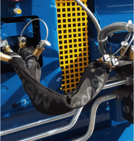
Hydraulic hose with safety trap and burst protection
